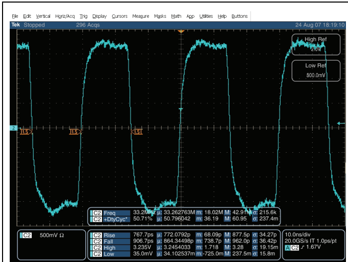
Slew_Rise & Slew_Fall
