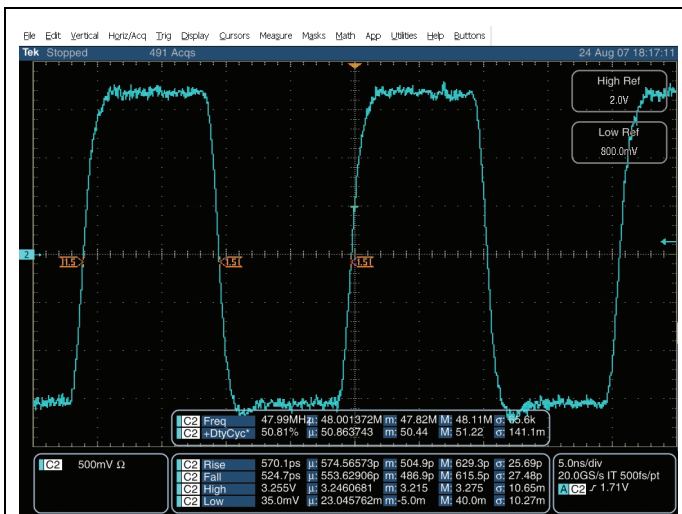
Slew_Rise & Slew_Fall
